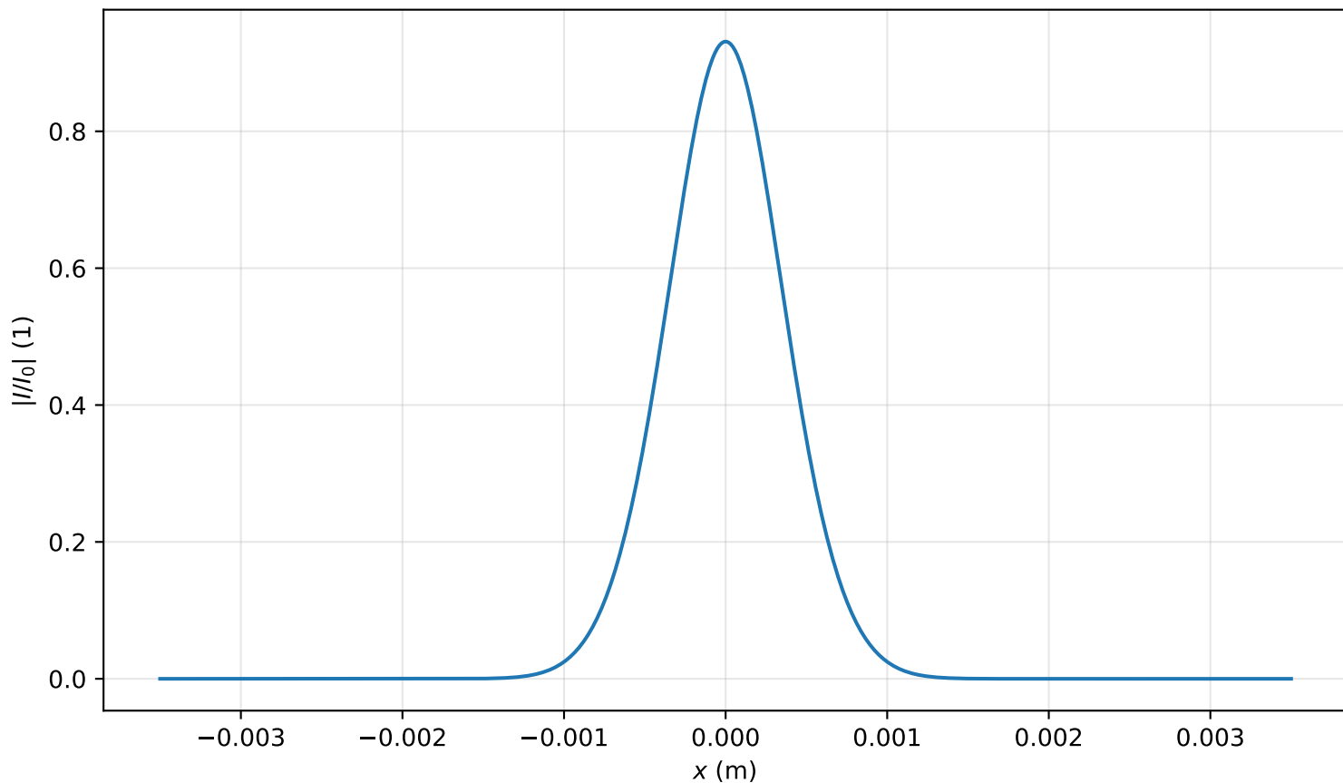
Intensity profile I(x, y = 0, z = 0.796m)/I_0 , P_{in}=0.2P_{cr} , artificial time
